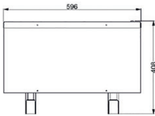
Side view outside unit :
