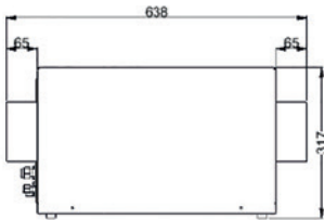
Side view evaporator unit :
