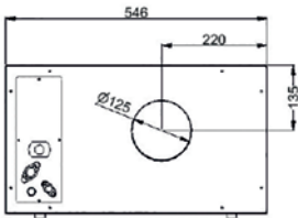
Thermostat front view :
