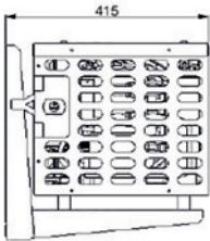
Front view evaporator unit :
