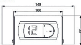
Thermostat side view :
